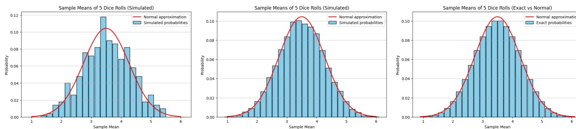
Figure: The histogram of the sample mean of a roll of 5 dice were plotted over 500, 10000, \infty simulations.
